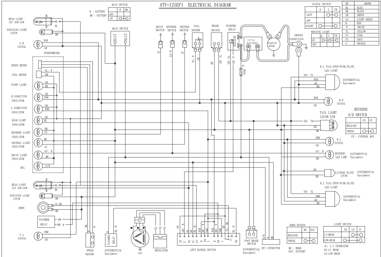
ATV-125EFI ELECTRICAL DIAGRAM
